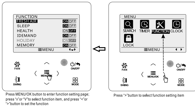
Figure 4-8 Function setting
