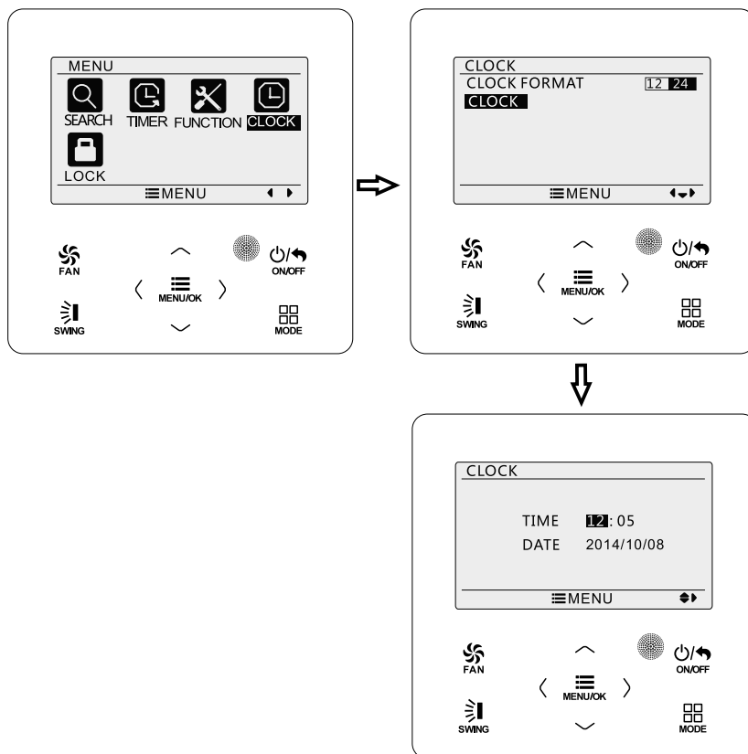
Figure 4-20 Clock setting
